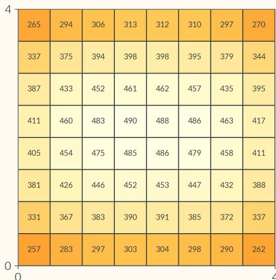
PPFD at 60" Mounting Height, 4 FIXTURES
