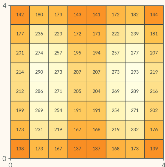
PPFD at 60" Mounting Height, 2 FIXTURES
